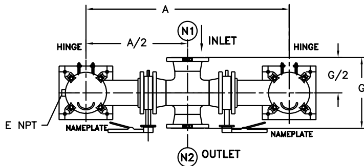
ASSEMBLY PLAN VIEW
