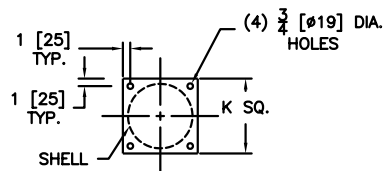
BASE PLATE DETAIL
