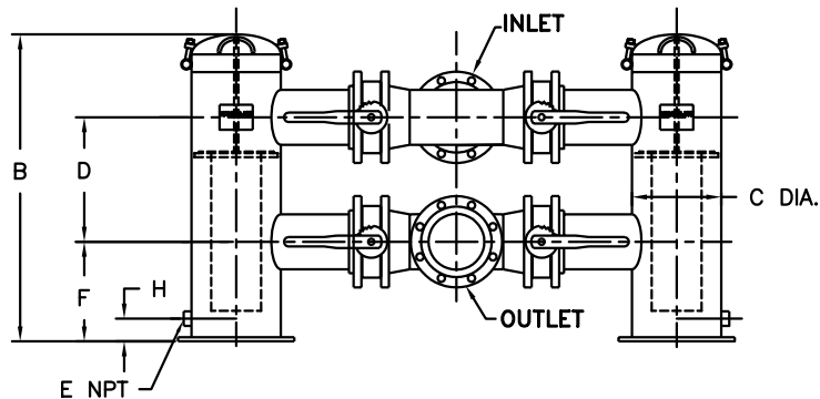
ASSEMBLY ELEVATION VIEW
